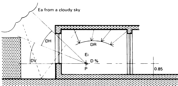
31 Daylight and internal area illuminance at point P
